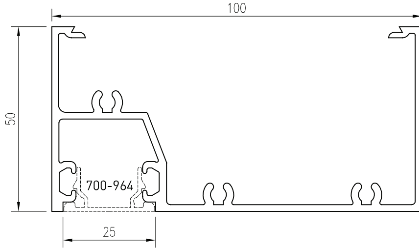
700-100 Frame - Face Glaze I_{xx} = 761.18 \times 10^3 \text{ mm}^4
