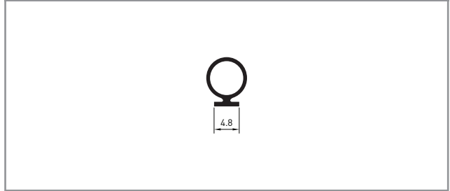
04-108 – Glazing Wedge
