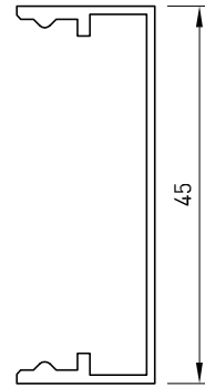
700-900 Cover Cap I_{xx} = 2.80 \times 10^3 \text{ mm}^4
