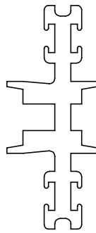
700-921 Clamp Bar I_{xx} = 2.20 \times 10^3 \text{ mm}^4
