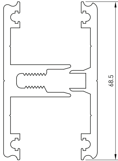
600-860 * Glazing Base I_{xx} = 21.8 \times 10^3 \text{ mm}^4
