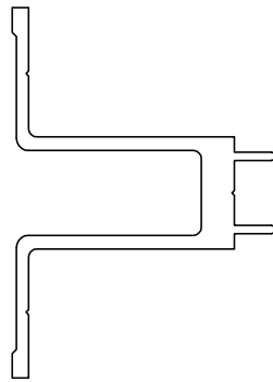
700-906 Glazing Base - IGU I_{xx} = 20.67 \times 10^3 \text{ mm}^4
