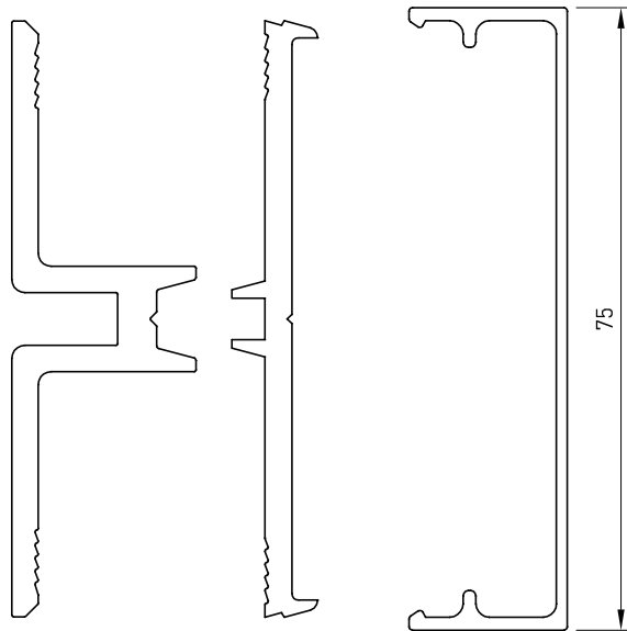
600-477 * Glazing Base I_{xx} = 13.68 \times 10^3 \text{ mm}^4
