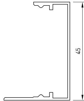
700-922 Cover Cap I_{xx} = 7.62 \times 10^3 \text{ mm}^4
