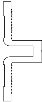
700-905 Glazing Base I_{xx} = 6.60 \times 10^3 \text{ mm}^4
