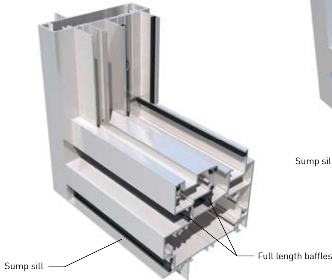
Optional Sliding Window with Sump Sill
