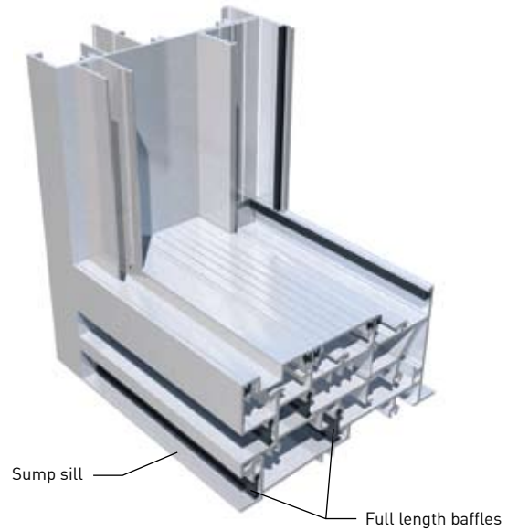
Optional Stacking Window with Sump Sill
