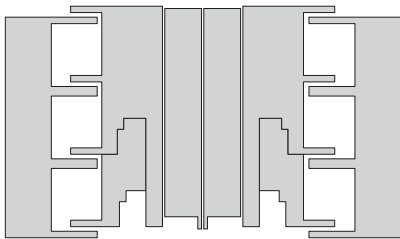
09-109 – Corner Stake (Flydoor)
