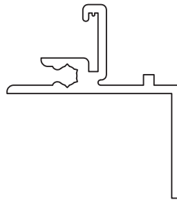
700-933 * Adaptor - 413 System Sash
